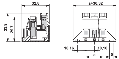
Dimensioned drawing
