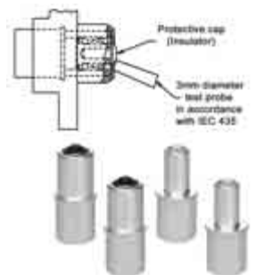
3 mm Diameter Test Probe in Accordance with IEC 435 Protective Cap (insulator)
