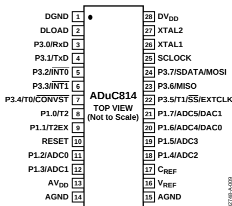
Figure 2. Pin Configuration
