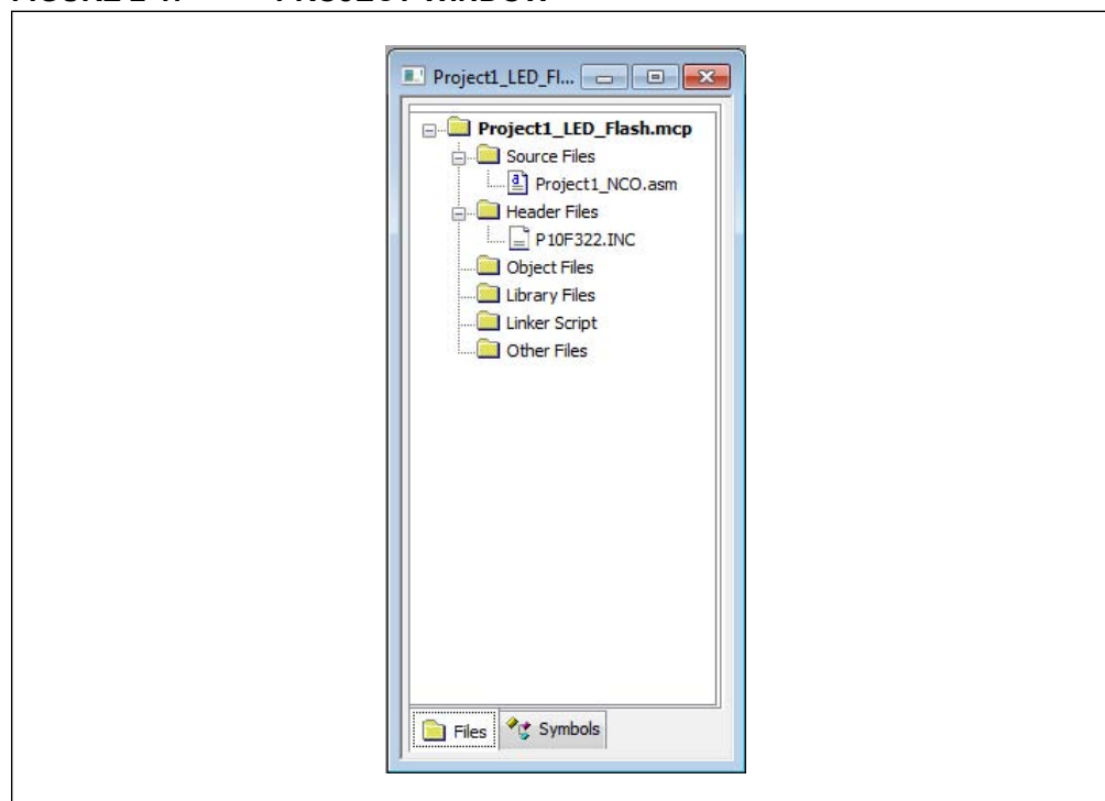
FIGURE 2-1: PROJECT WINDOW
