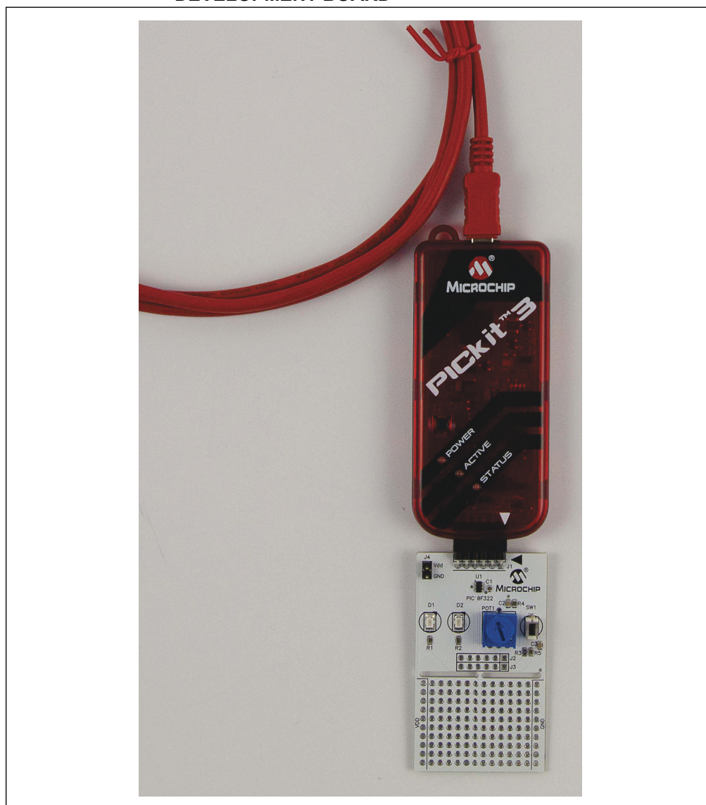
FIGURE 1-4: CONNECTING THE PICKIT™ 3 TO THE PIC10(L)F32X DEVELOPMENT BOARD
