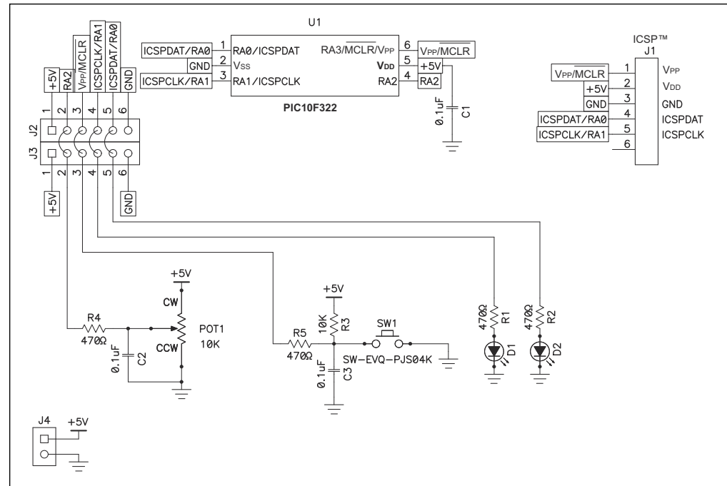
FIGURE A-1: PIC10(L)F32X DEVELOPMENT BOARD HARDWARE SCHEMATIC DIAGRAM
