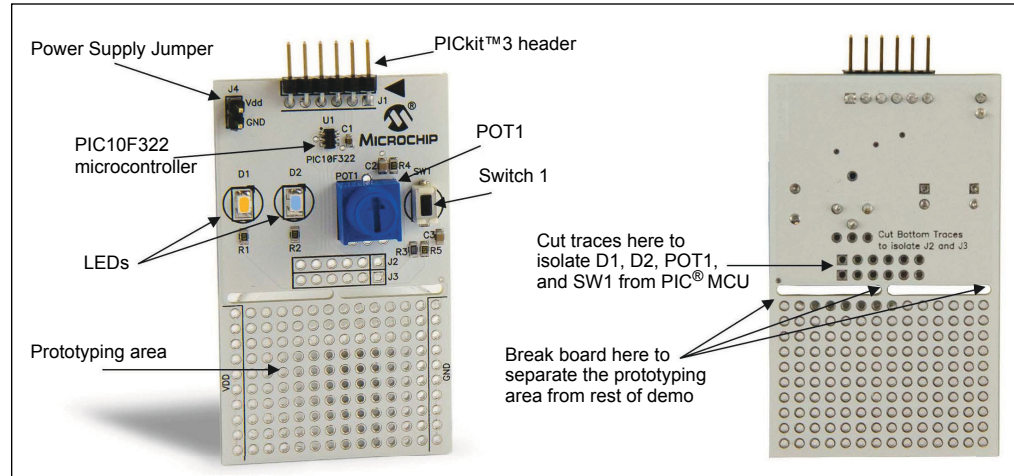
FIGURE 1-2: PIC10(L)F32X DEVELOPMENT BOARD HARDWARE LAYOUT
