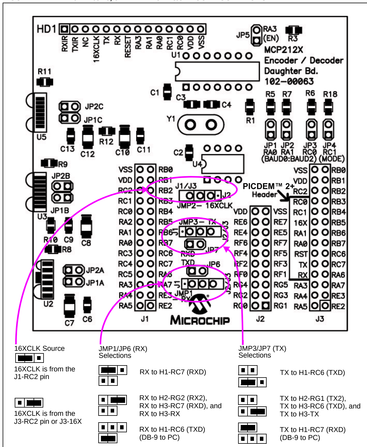
FIGURE 2-2: JMP1/JMP6, JMP2 AND JMP3/JMP7 CONFIGURATIONS
