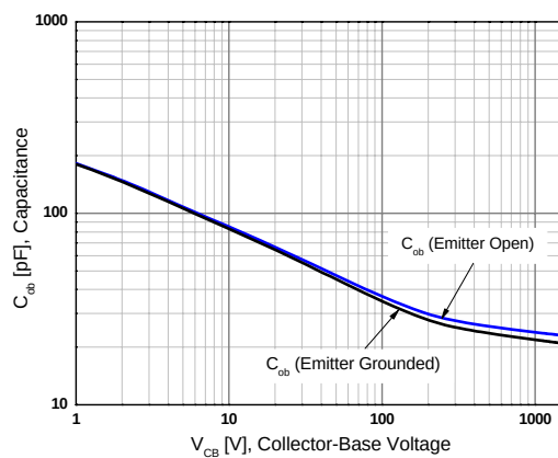
Figure 8. Capacitance
