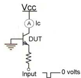
Fig4. FBSOA
