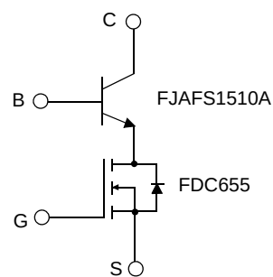
Figure 3. ESBC Configuration**
