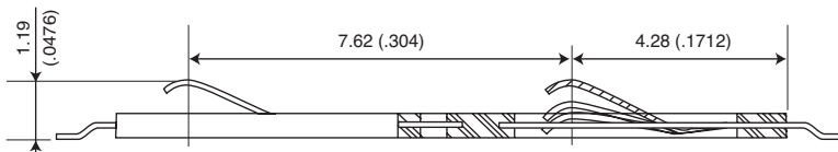
Connector Profile (Ref.)
