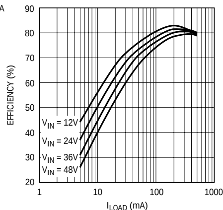
Figure 4b. P_{OUT}/P_{IN} Efficiency
