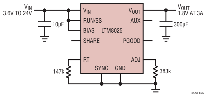
1.8V Step-Down Converter
