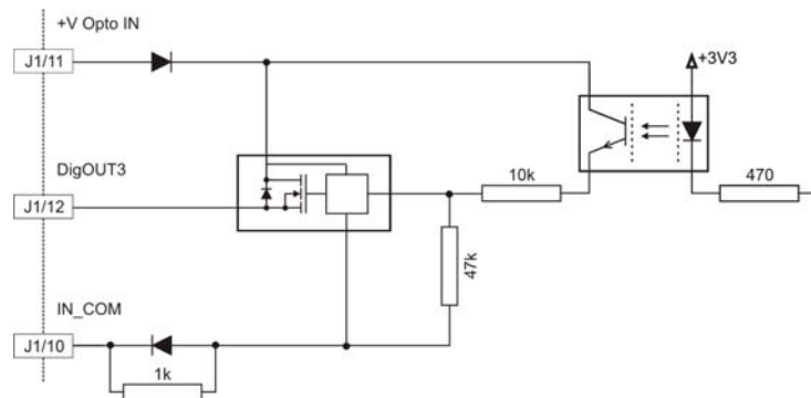
Figure 4-12 DigOUT3 Circuit – (analogously valid also for DigOUT4)
