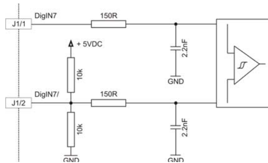
Figure 4-10 DigIN7 “Differential” Circuit (analogously valid also for DigIN8)
