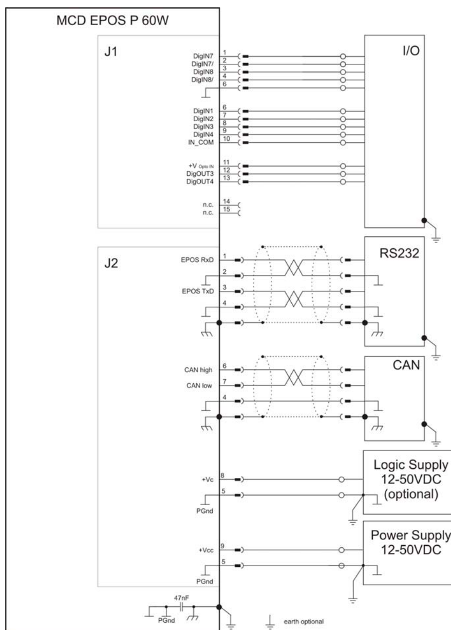
Figure 4-4 Wiring Diagram
