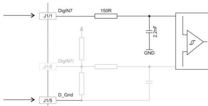
Figure 4-11 DigIN7 “Single-ended” Circuit (analogously valid also for DigIN8)
