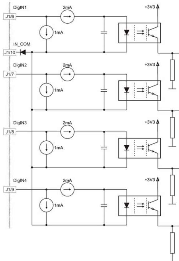
Figure 4-8 DigIN1...4 Circuit
