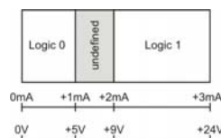
Figure 4-7 DigIN1...4 Logic Level
