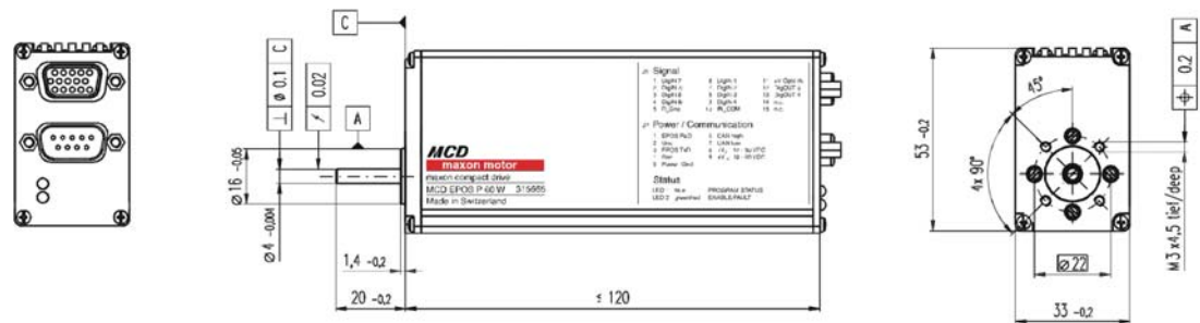
Figure 3-2 Dimensional Drawing [mm]
