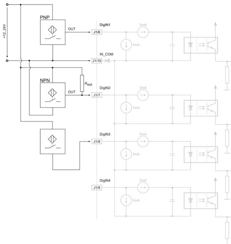
Figure 4-9 DigIN1...4 – Wiring Example for different Types of Proximity Switches
