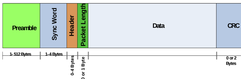
Figure 11. Packet Structure
