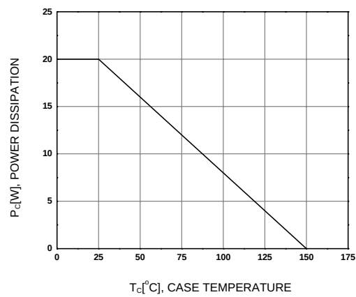
Figure 1. Power Derating
