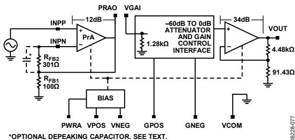
Figure 77. Simplified Block Diagram
