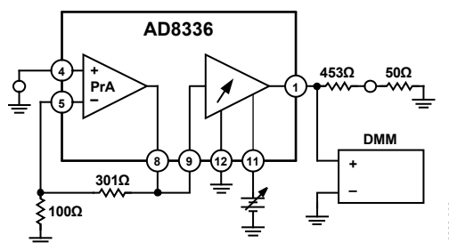
Figure 60. Offset Voltage
