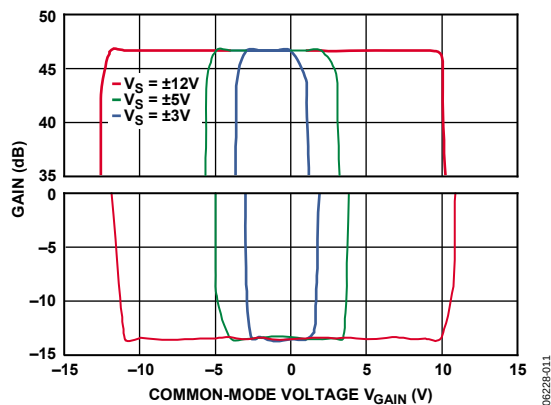
Figure 11. Gain vs. Common-Mode Voltage at V_{\text{GAIN}}
