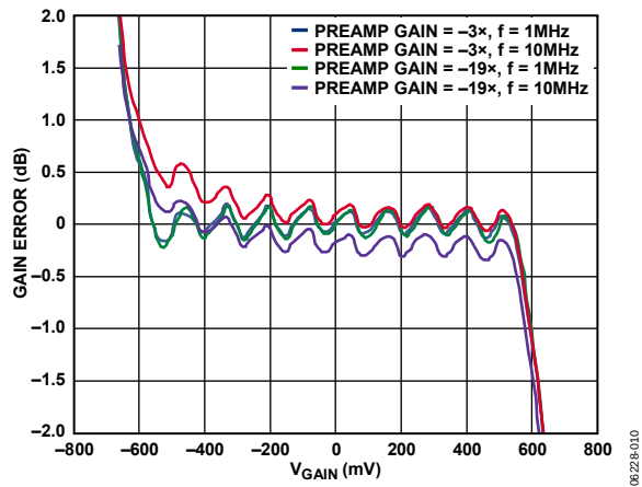
Figure 10. Gain Error vs. V_{\text{GAIN}} at 1 MHz and 10 MHz and for Inverting Preamp Gains of -3x and -19x (See Figure 56)
