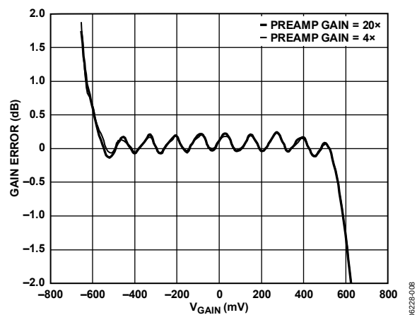
Figure 8. Gain Error vs. V_{\text{GAIN}} for Preamp Gains of 4\times and 20\times (See Figure 56)
