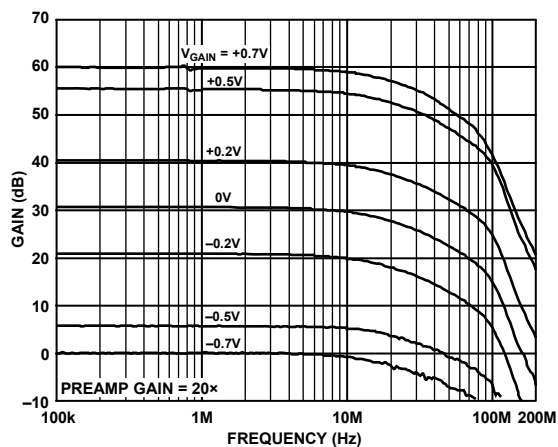
Figure 20. Frequency Response for Various Values of V_{GAIN} When the Preamp Gain is 20x (See Figure 57)
