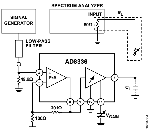
Figure 64. Harmonic Distortion
