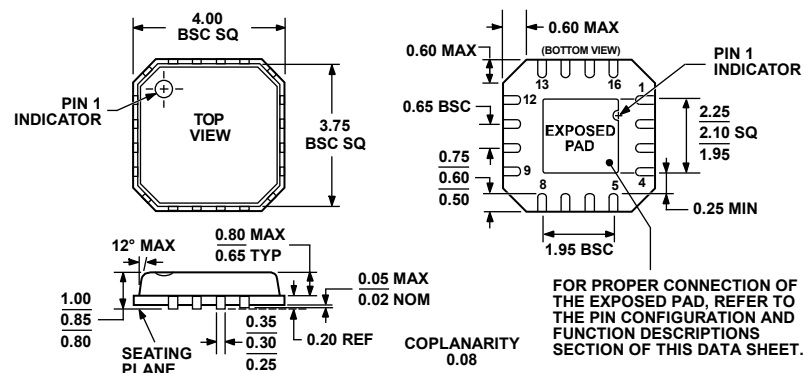
Figure 89. 16-Lead Lead Frame Chip Scale Package [LFCSP_VQ]
