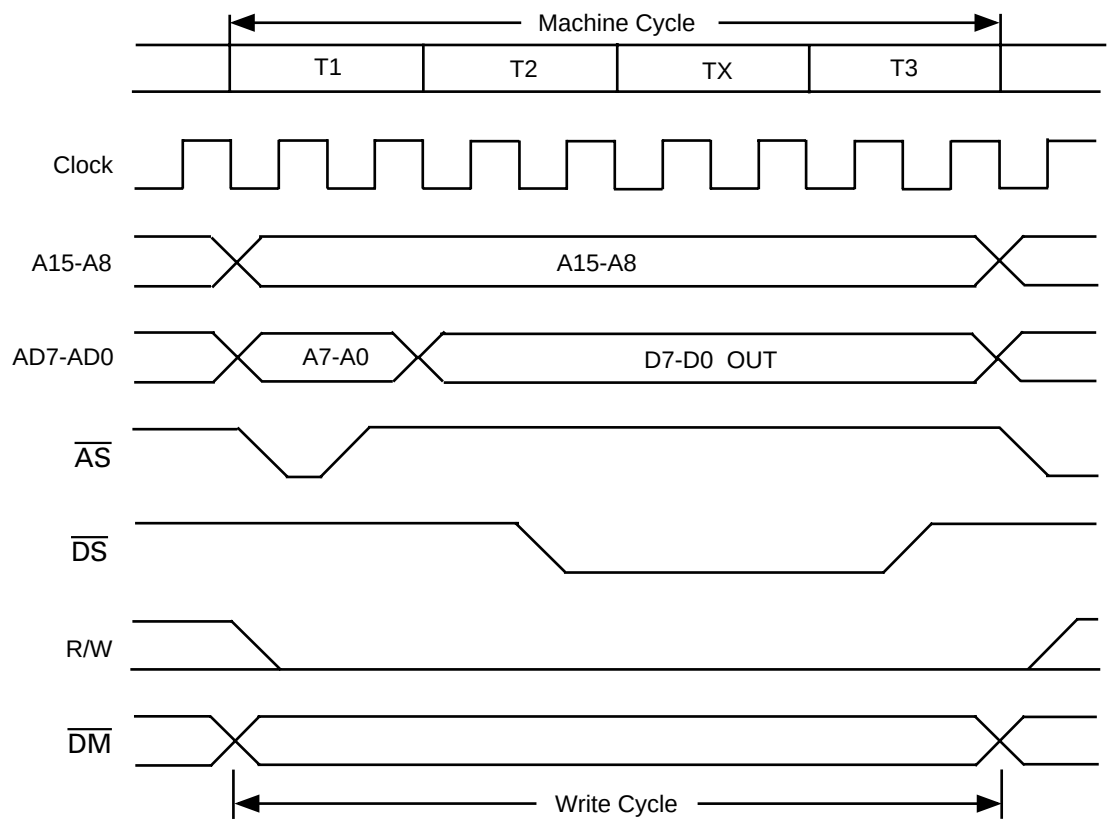
Figure 10-8. Extended External Memory Write Cycle
