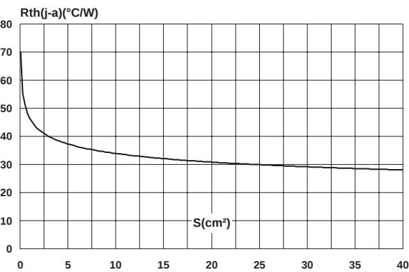
Fig. 10: Thermal resistance junction to ambient versus copper surface under tab (epoxy printed board FR4, Cu = 35μm) (STPS41L60CG only).
