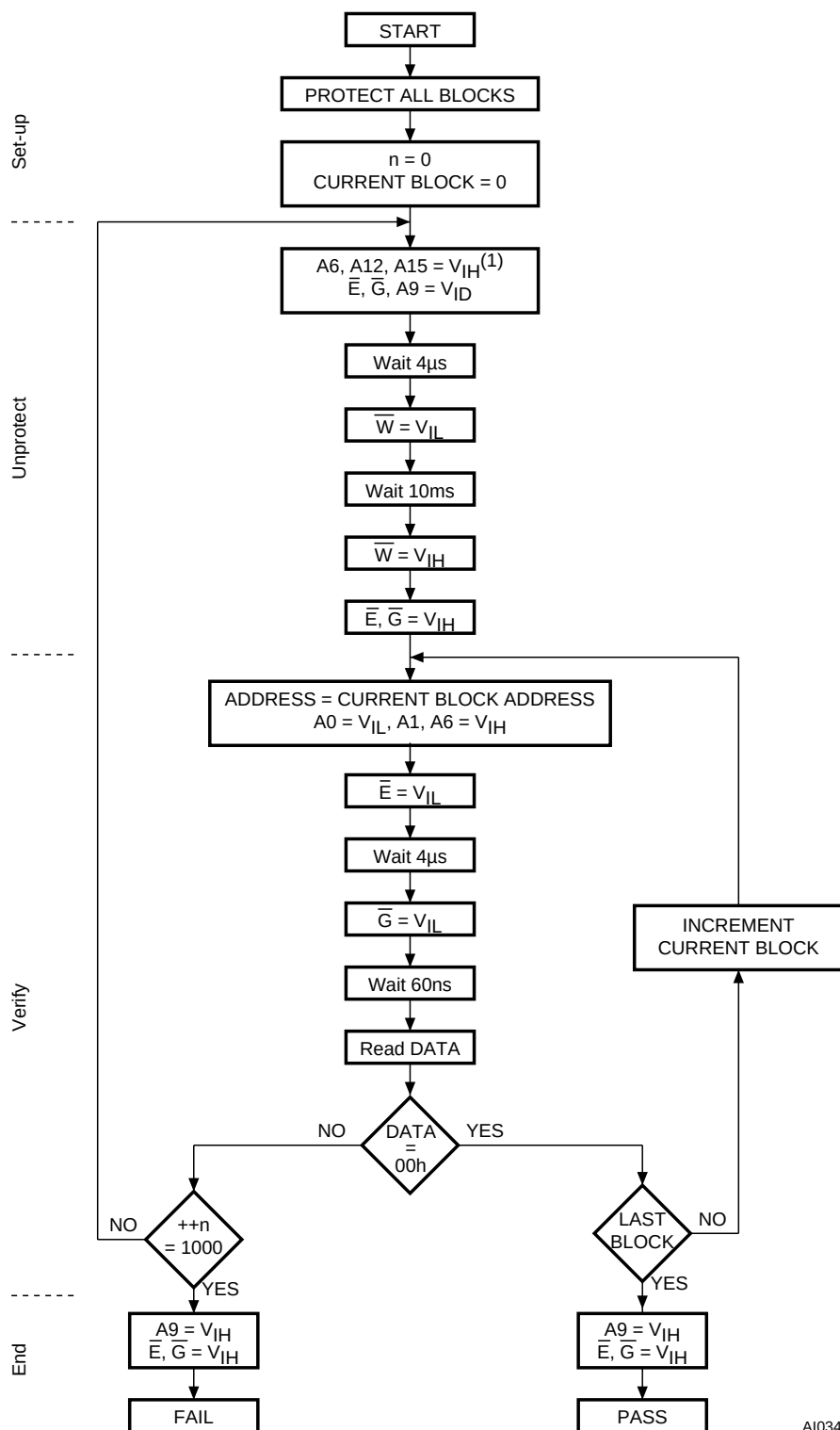
Figure 19. Programmer Equipment Chip Unprotect Flowchart
