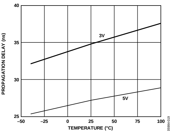
Figure 13. Propagation Delay vs. Temperature, C Grade
