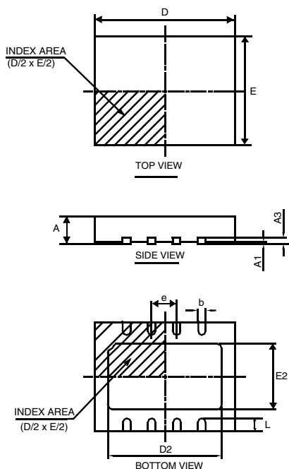
Figure 66. 8-Lead Very thin Fine pitch Dual Flat No-Lead Package
