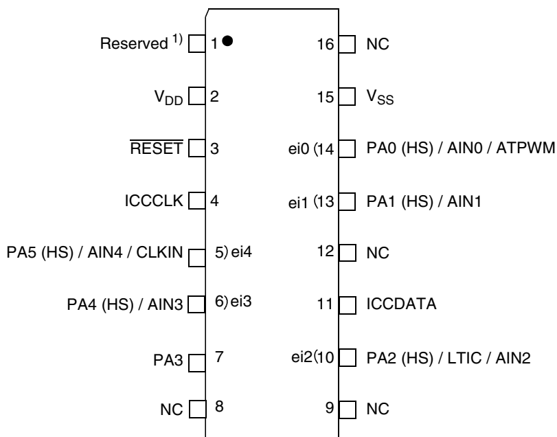
Figure 4. 16-pin package pinout (For development or tool prototyping purposes only. Package not orderable in production quantities.)
