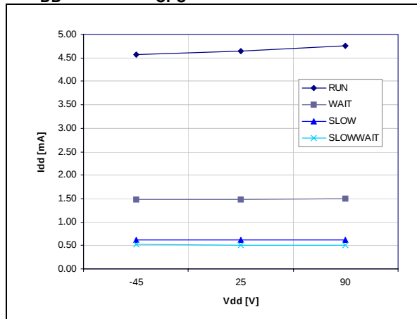
Figure 46. Typical I_{DD} vs. temperature at V_{DD} = 5V and f_{CPU} = 8MHz
