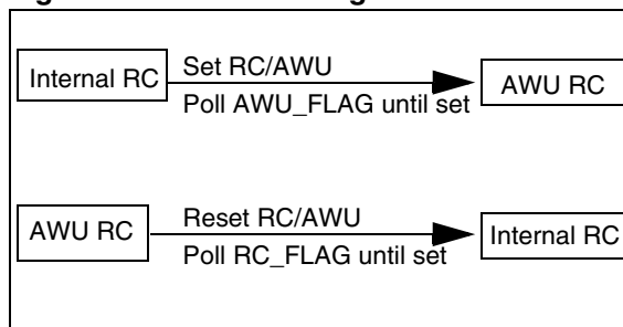
Figure 9. Clock Switching
