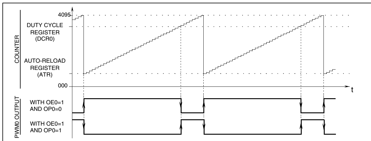
Figure 34. PWM Function
