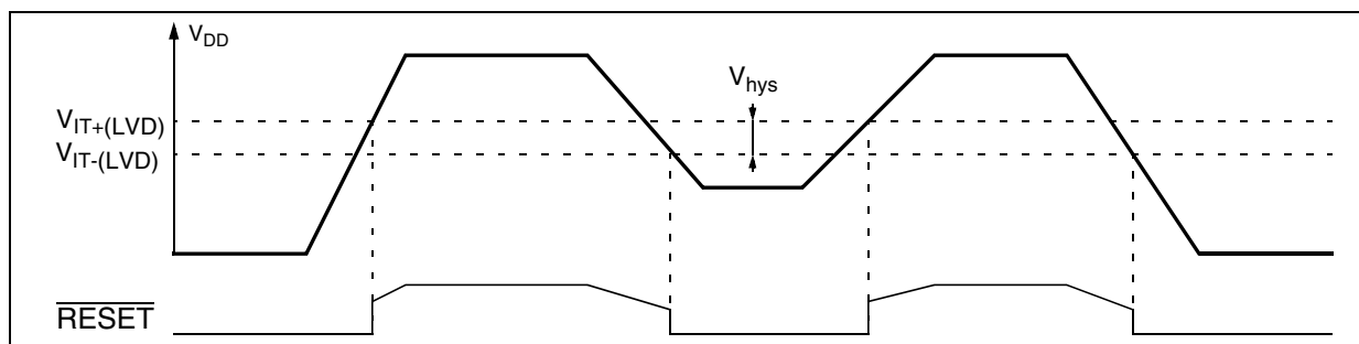
Figure 15. Low Voltage Detector vs Reset
