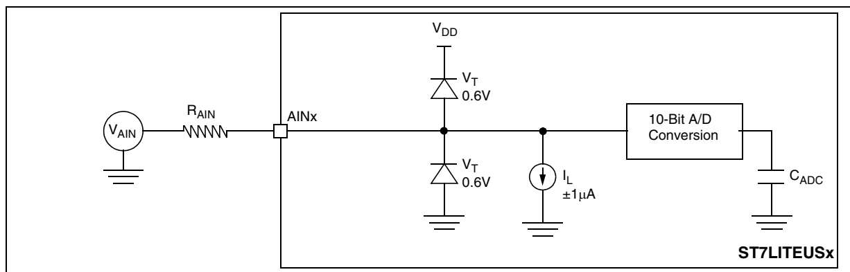
Figure 64. Typical Application with ADC
