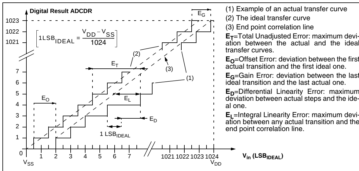
Figure 65. ADC Accuracy Characteristics
