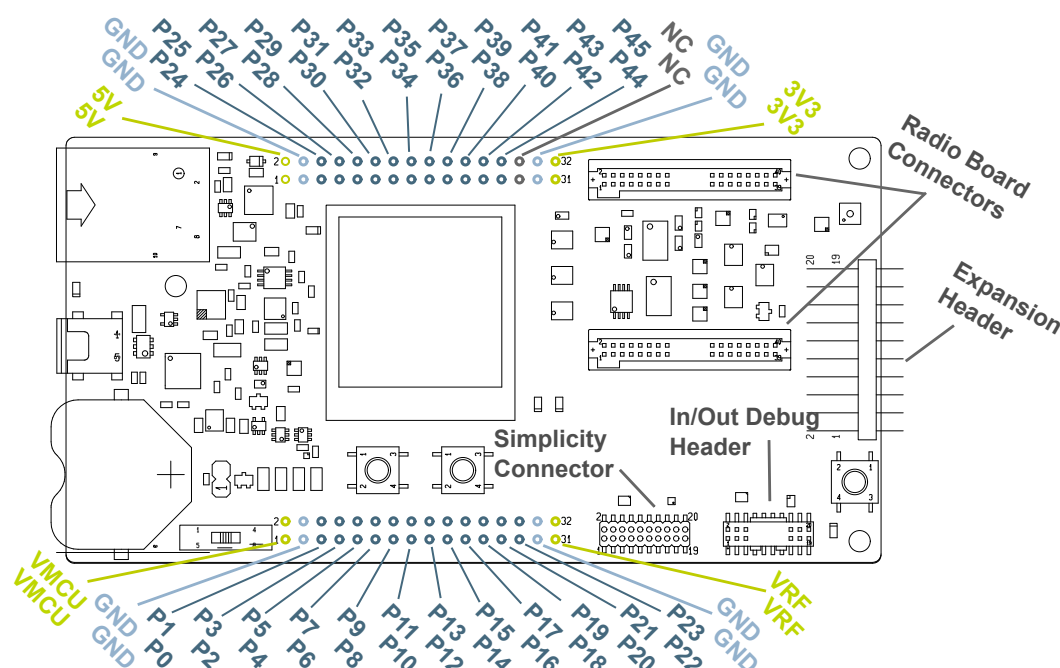
Figure 9.1. Connector layout
