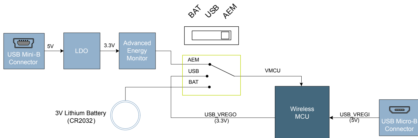
Figure 4.1. WSTK6220 Power Switch
