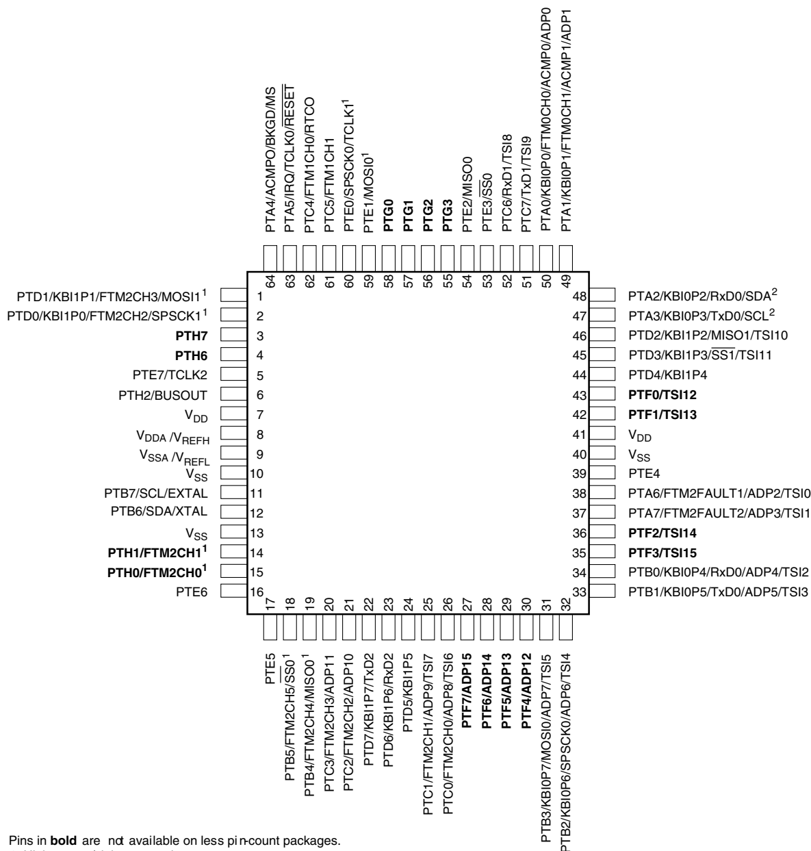
Figure 17. MC9S08PT60 64-pin QFP and LQFP package
