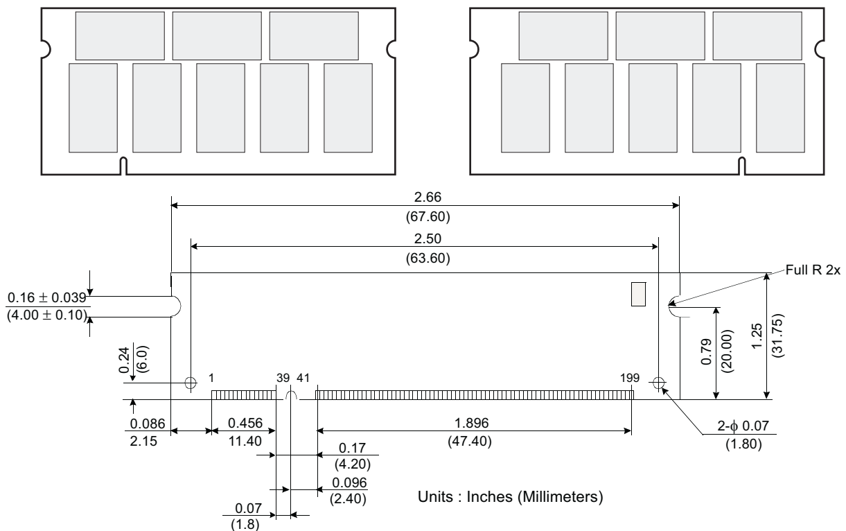
Figure 1: KVR400X64SC3A/1G 200-Pin SODIMM
