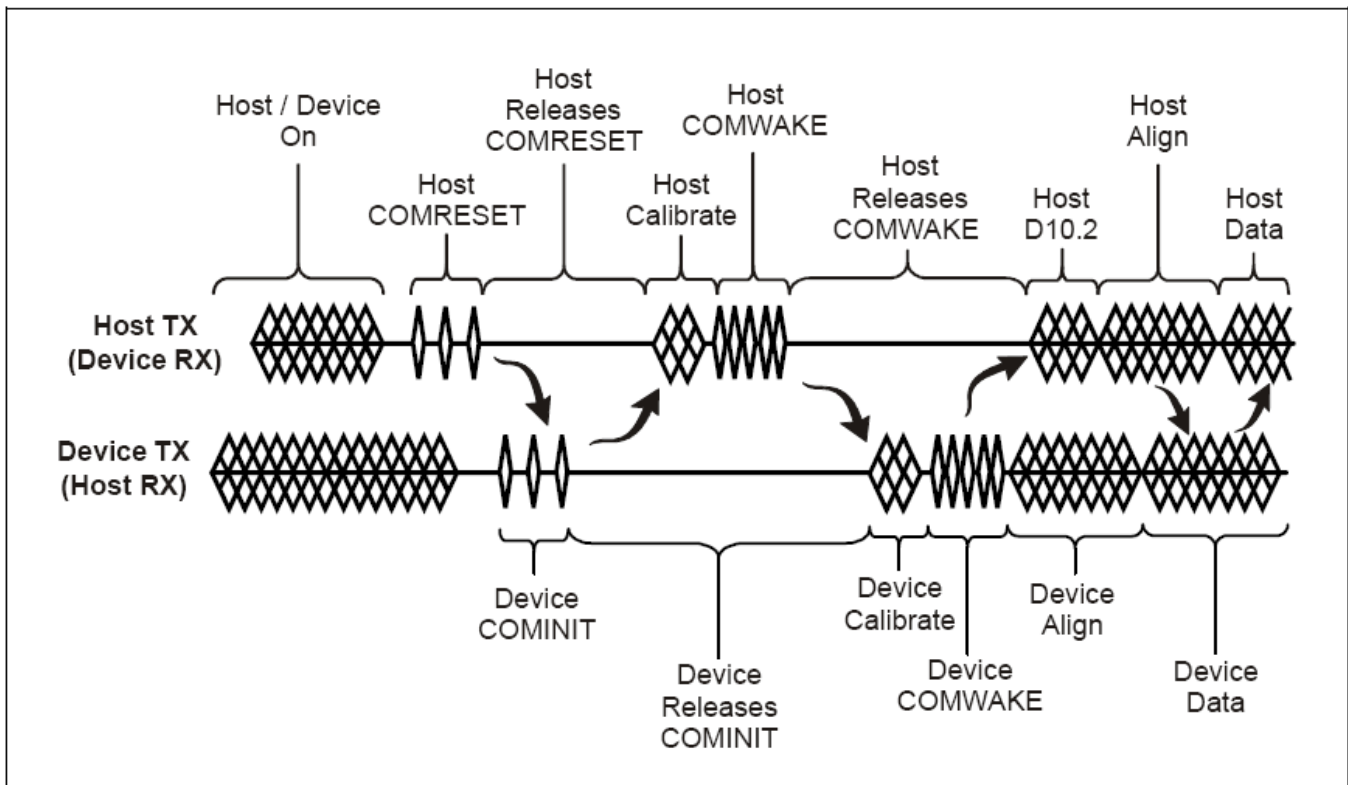
Figure 5: Comreset sequence
