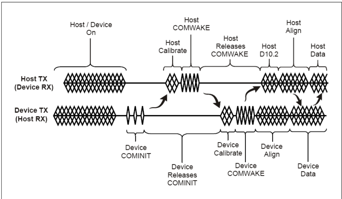
Figure 6: cominit sequence
