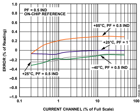
Figure 6. Error as a % of Reading over Temperature with On-Chip Reference (PF = 0.5 IND)
