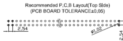
Dimension L
