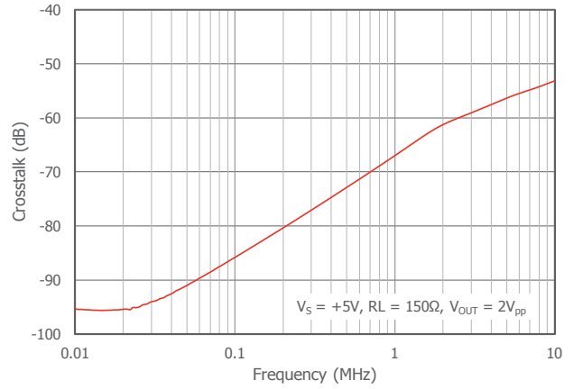
Crosstalk vs Frequency
