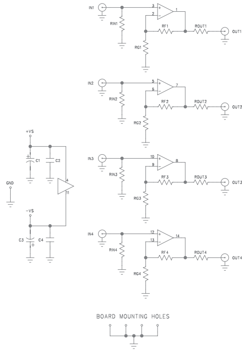
Figure 18. CEB018 Schematic
