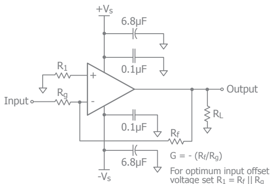
Figure 2. Typical Inverting Gain Circuit
