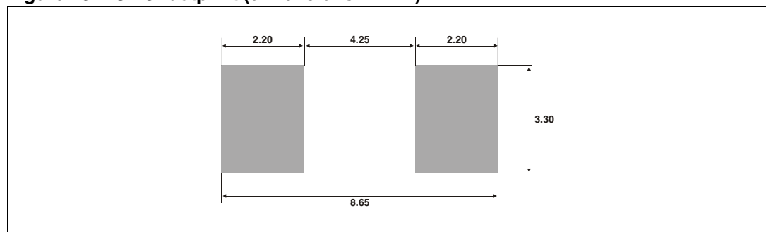
Figure 20. SMC footprint (dimensions in mm)
