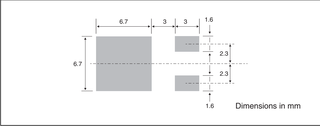
Figure 18. DPAK footprint
