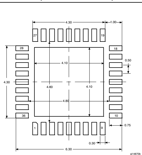
Figure 41. Recommended footprint (dimensions in mm) (1)(2)(3)
