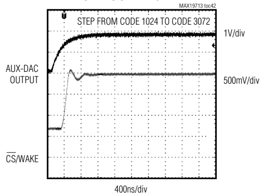
AUX-DAC SETTLING TIME
