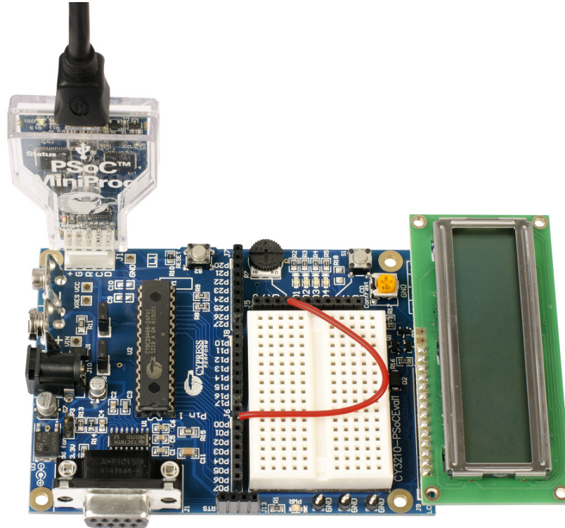
Figure 5-27. Connect MiniProg1 to Board
