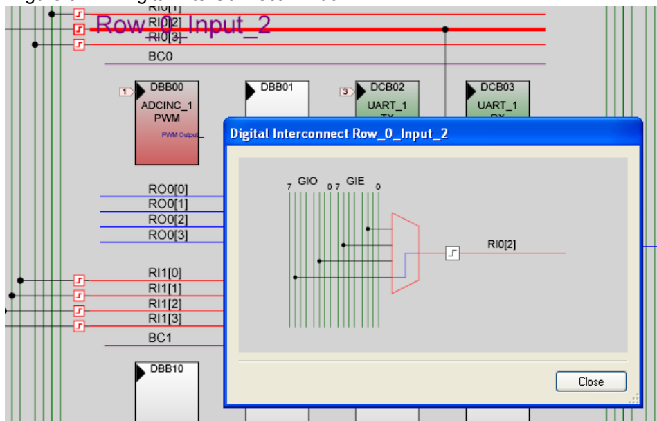
Figure 5-17. Digital InterConnect Window
