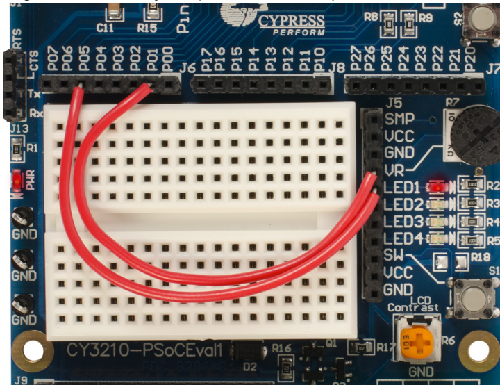
Figure 5-47. Verify Output: Code Example 4
