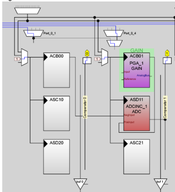
Figure 5-10. PGA User Module Placement
