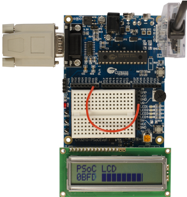
Figure 5-34. Verify Output on LCD
