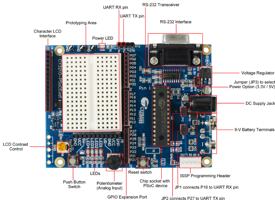
Figure 4-2. CY3210-PSoCEVAL1 Evaluation Board
