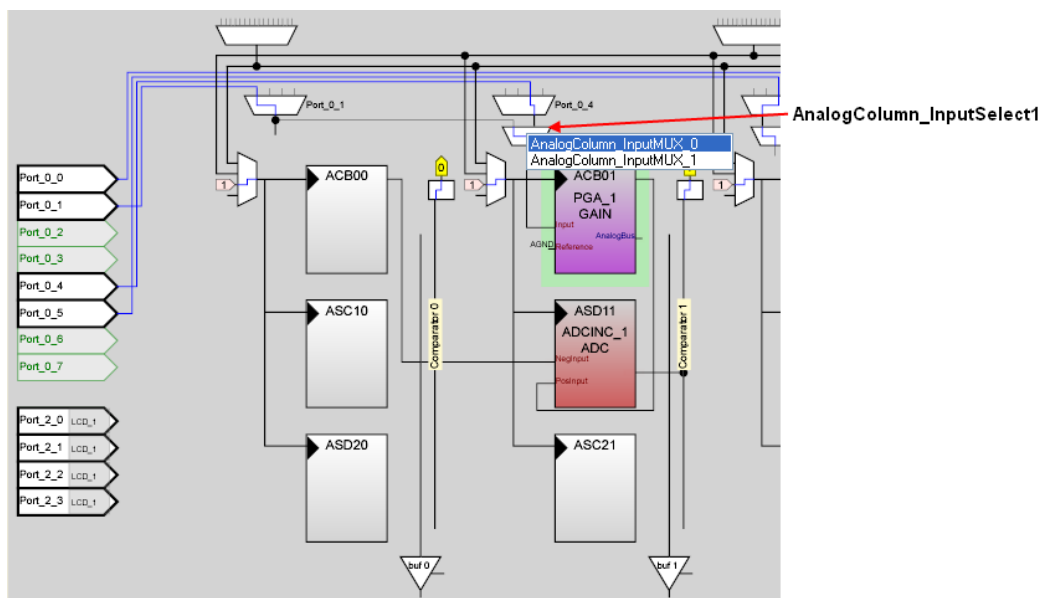
Figure 5-12. Connecting PGA to Port Pin
