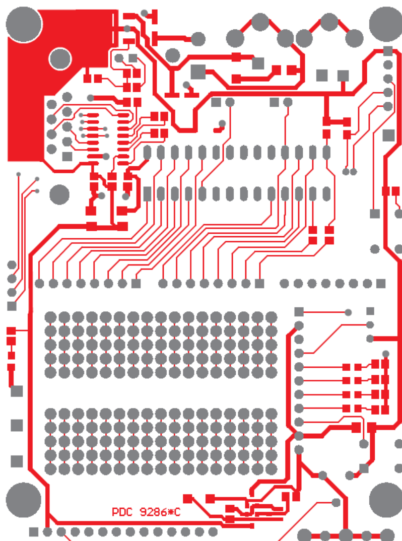
Figure A-1. Top Copper Layer
