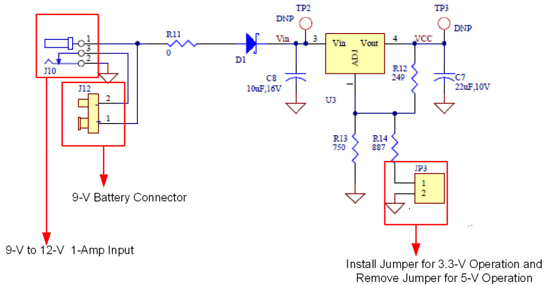
Figure 4-3. Power Supply Schematic
