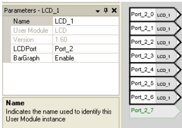
Figure 5-14. LCD User Module Placement
