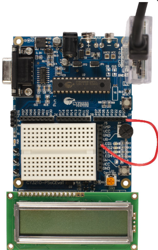
Figure 5-42. Hardware Connection: Code Example 3
