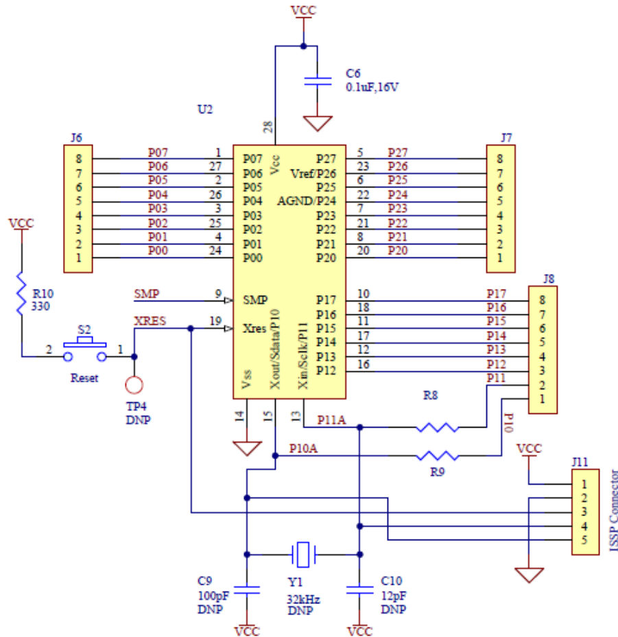
Figure 4-8. Prototyping Area Schematic
