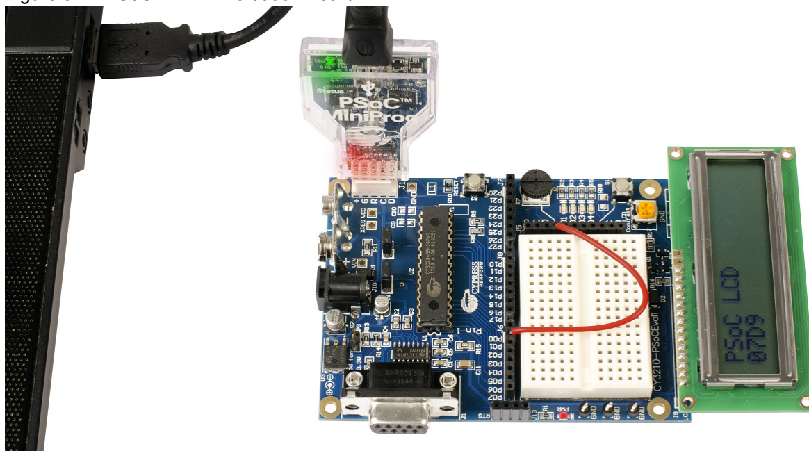
Figure 3-1. PSoCEVAL1 Evaluation Board
