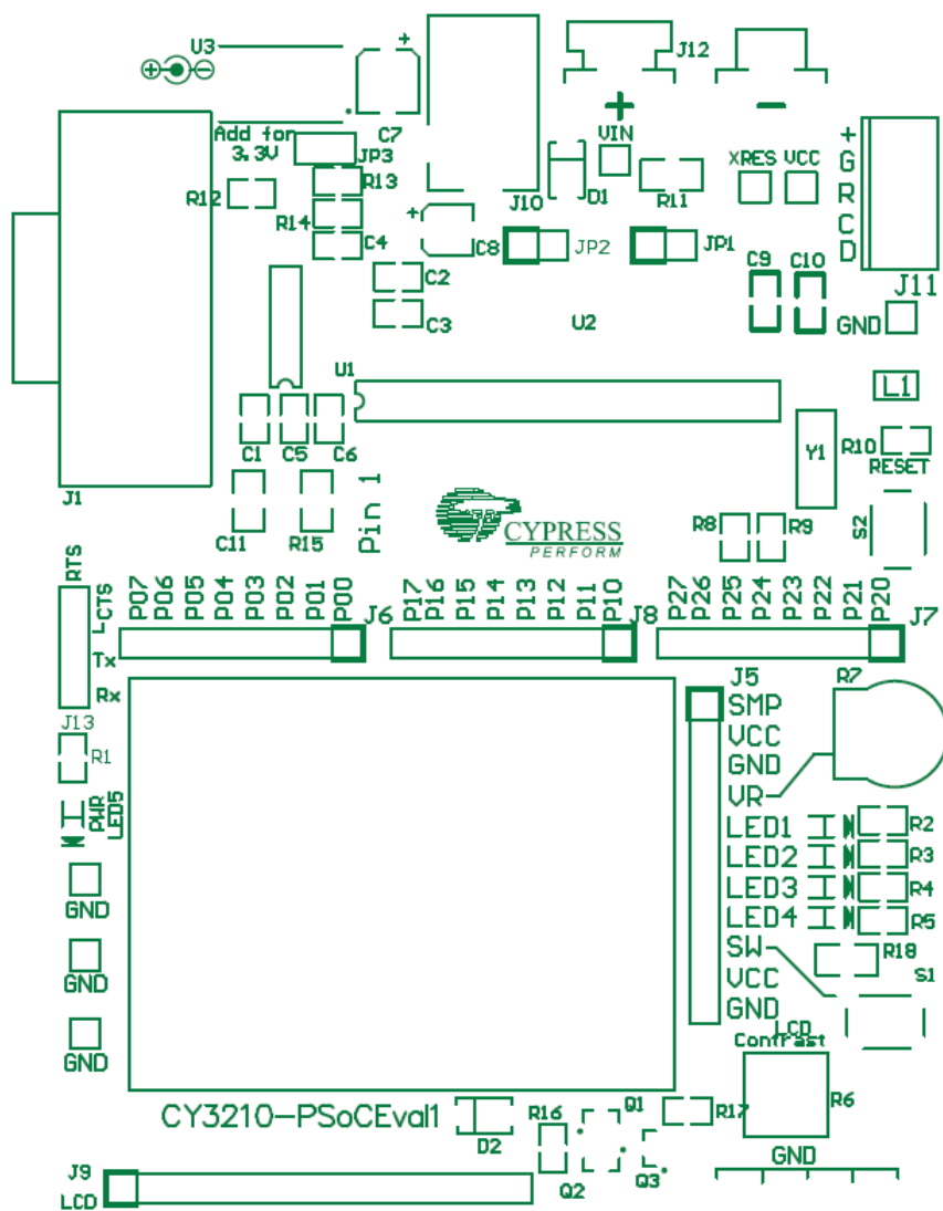
Figure A-3. Top Overlay
