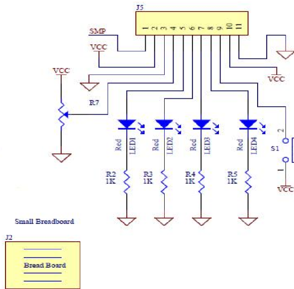
Figure 4-9. Prototyping Area Schematic
