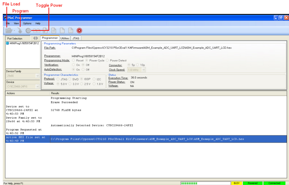
Figure 3-3. PSoC Programmer Screen
