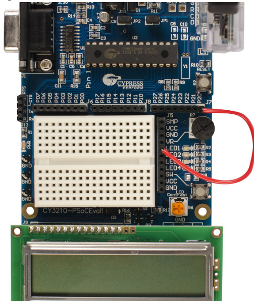
Figure 5-54. Hardware Connection: Code Example 6
