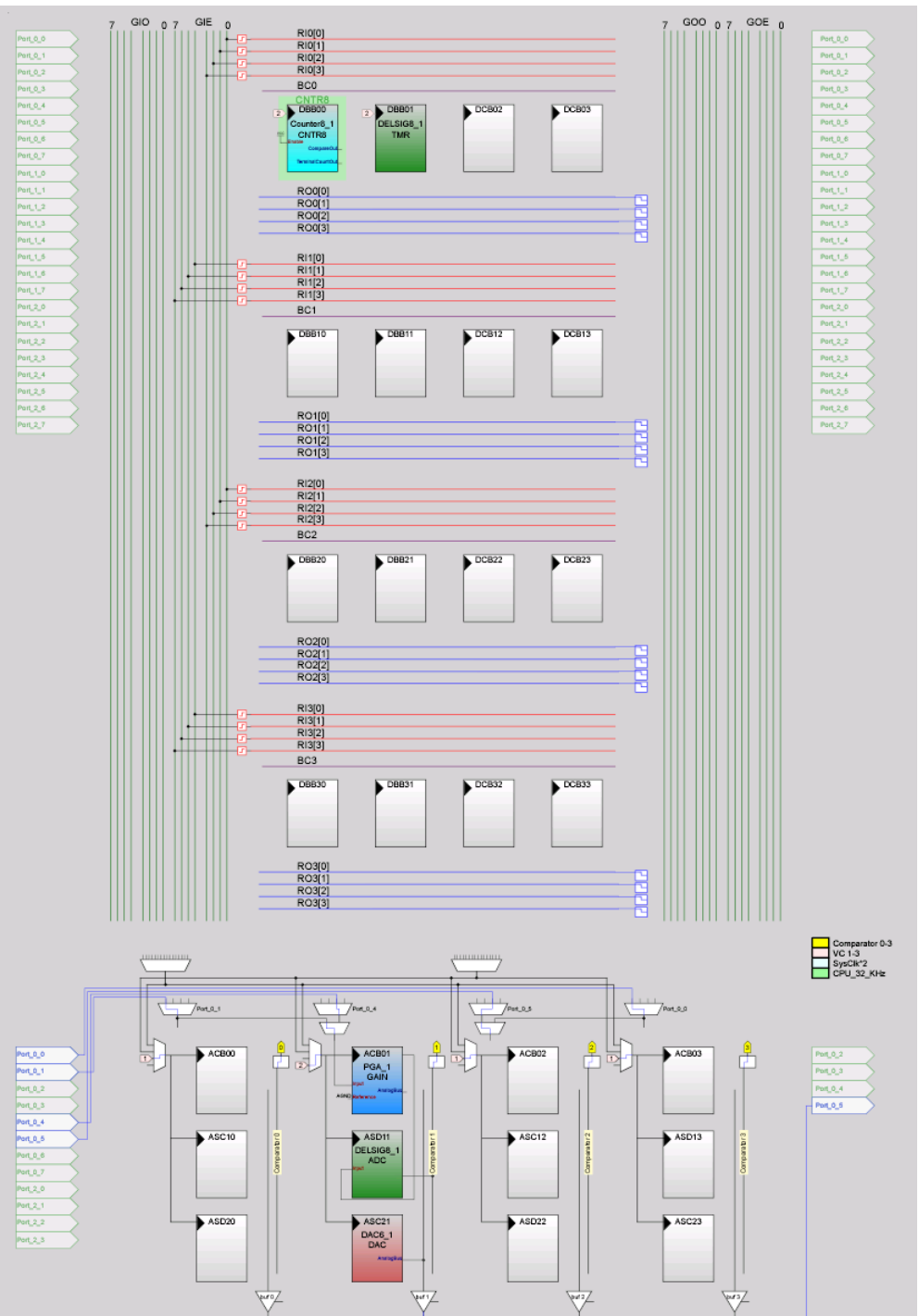
Figure 5-44. Device Configuration to Output a Sine Wave
