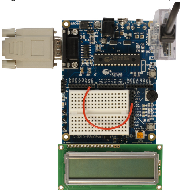
Figure 5-37. Hardware Connection: Code Example 2
