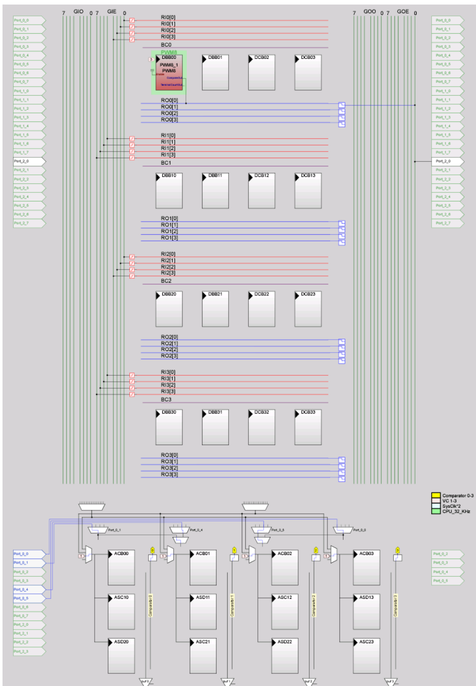
Figure 5-41. Device Configuration to Blink an LED
