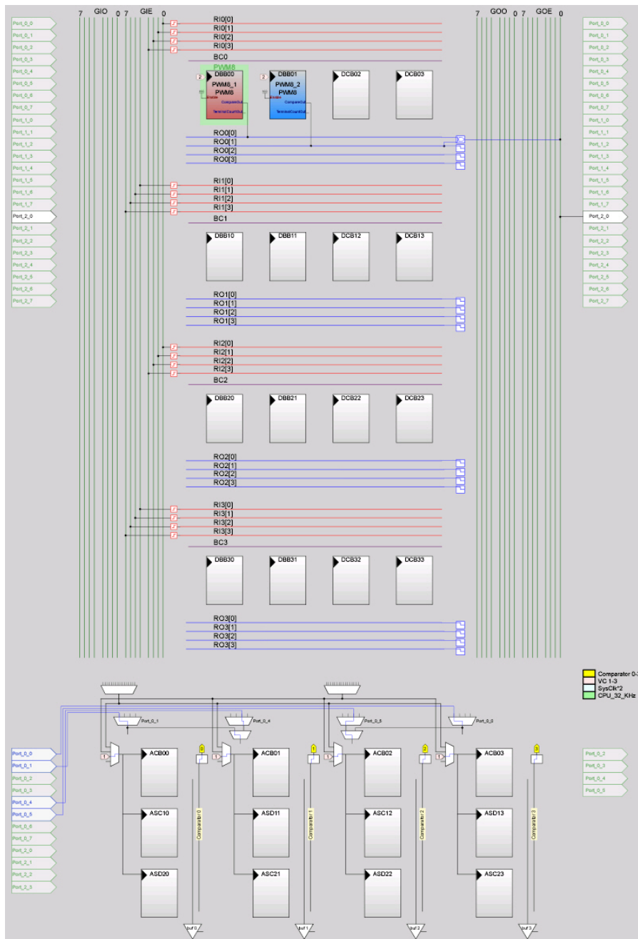
Figure 5-53. Device Configuration to Combine PWMs using Output Logic
