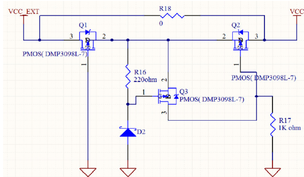
Figure 4-4. Protection Circuit
