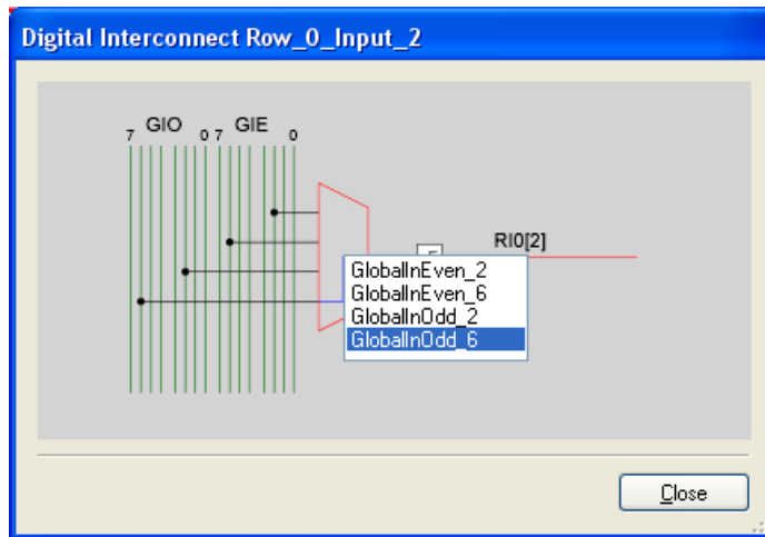
Figure 5-18. Configure Row_0_Input_2 to GlobalInOdd_6
