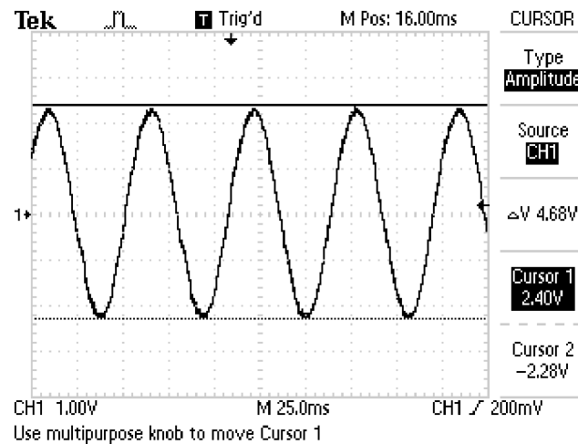
Figure 5-46. Output Sine Wave
