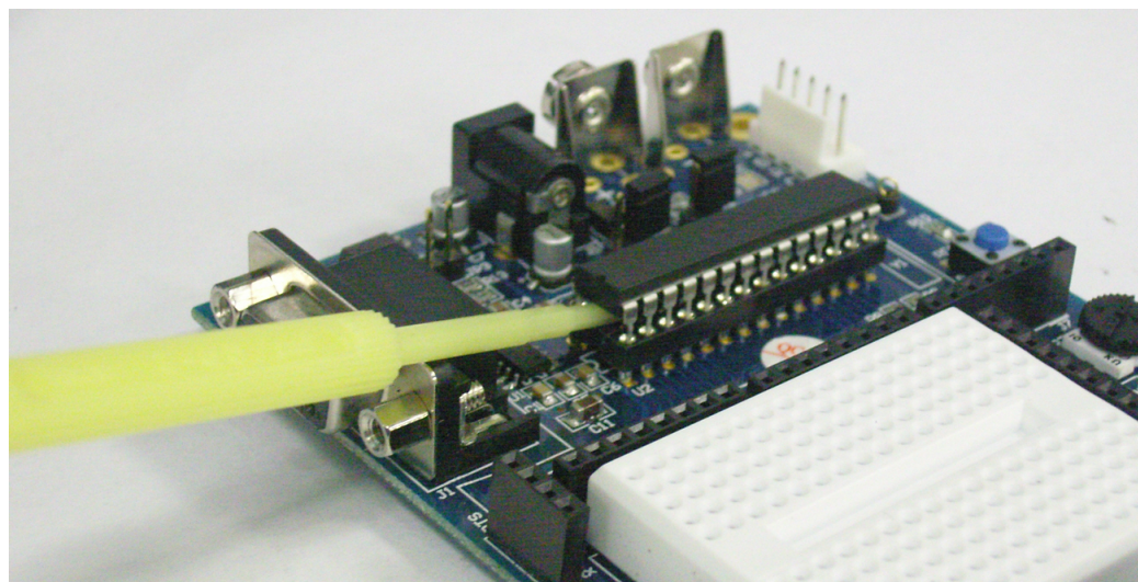
Figure A-5. Lift IC - Other Side
