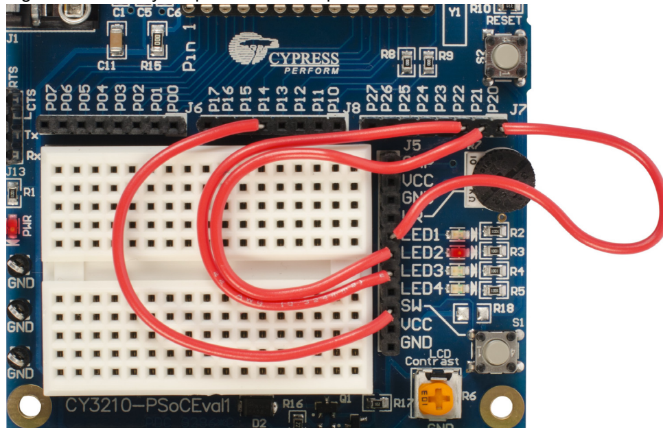
Figure 5-52. Verify Output: Code Example 5
