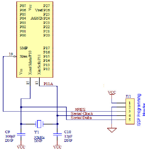
Figure 4-6. Programming Interface Schematic
