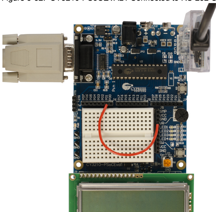
Figure 5-32. CY3210-PSocEVAL1 Connected to RS-232 Cable
