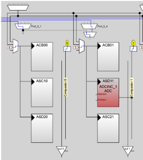
Figure 5-8. ADCINC User Module Placement
