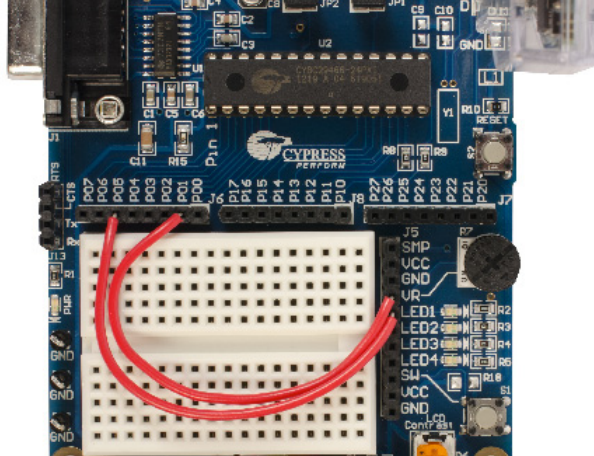
Figure 5-45. Hardware Connections: Code Example 4
