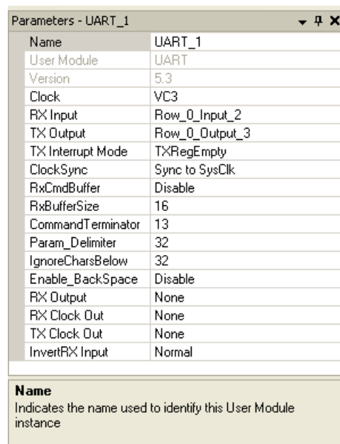
Figure 5-15. UART User Module Properties
