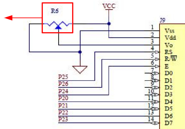
Figure 4-10. LCD Interfacing Schematic
