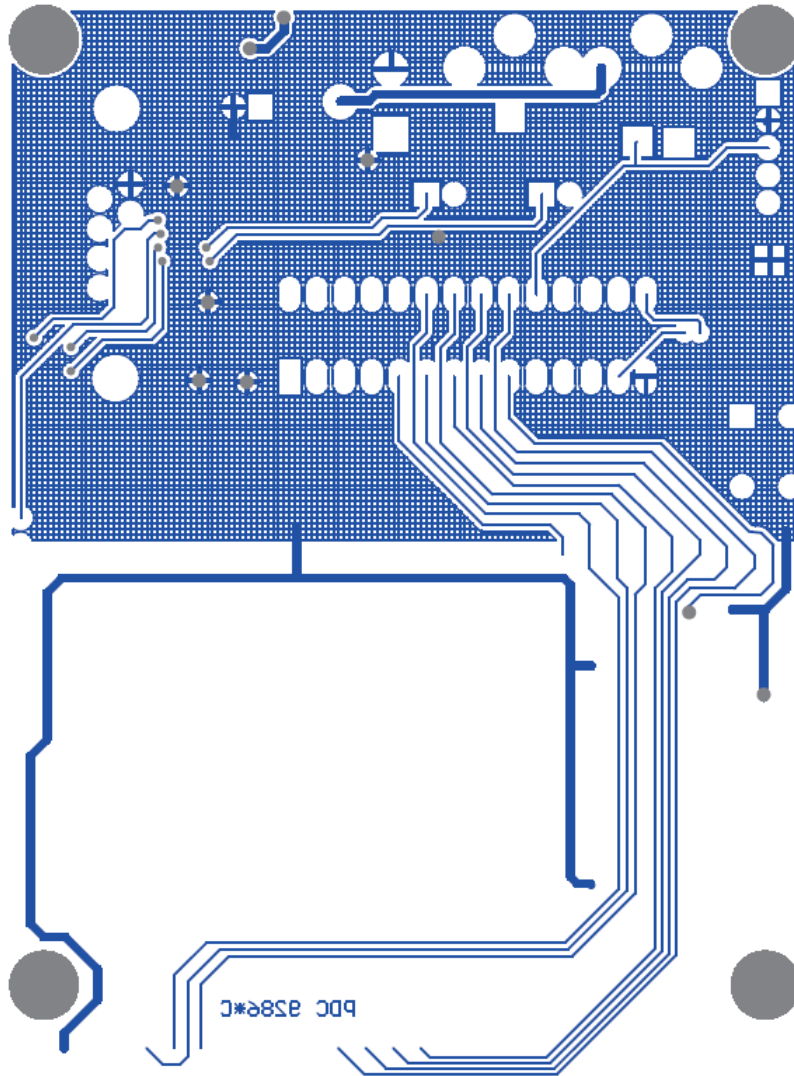
Figure A-2. Bottom Copper Layer
