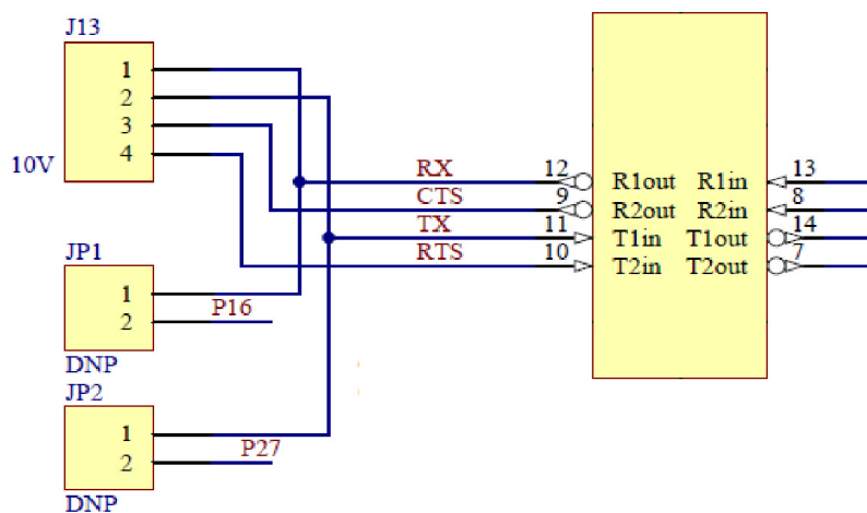
Figure 4-5. Jumper Settings
