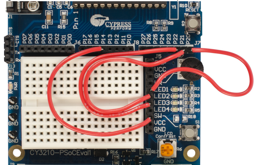
Figure 5-51. Hardware Connection: Code Example 5
