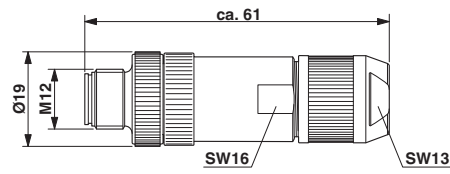
Dimensioned drawing
