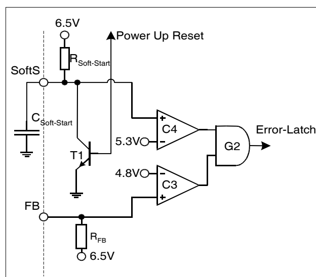
Figure 22 FB-Detection
