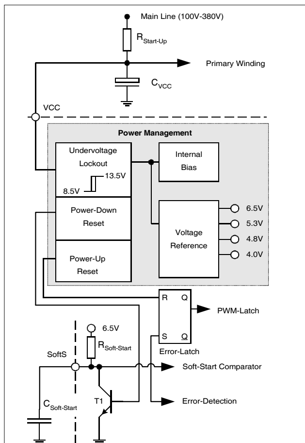
Figure 6 Power Management
