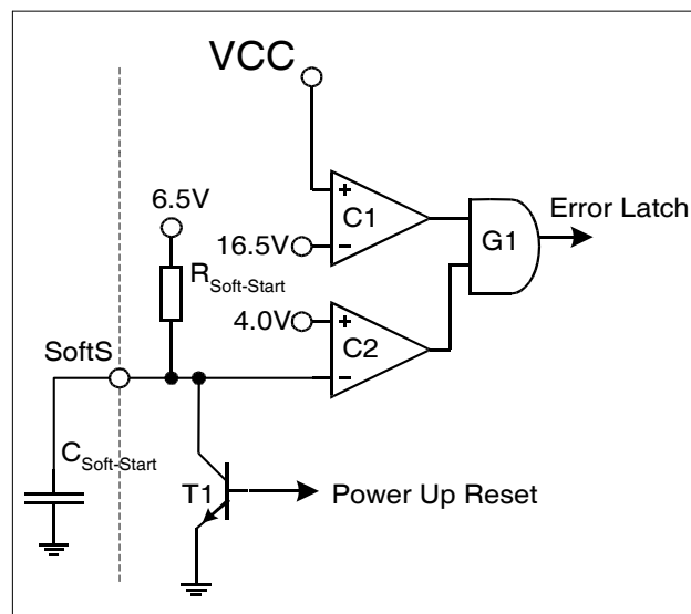
Figure 24 Overvoltage Detection
