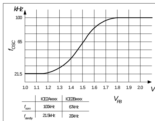
Figure 15 Frequency Dependence
