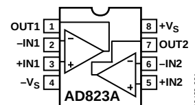
Figure 1. 8-Lead SOIC
