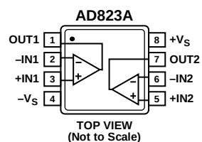
Figure 2. 8-Lead MSOP
