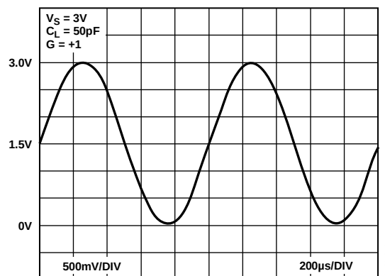
Figure 3. Output Swing, +V_S = +3 V, G = +1
