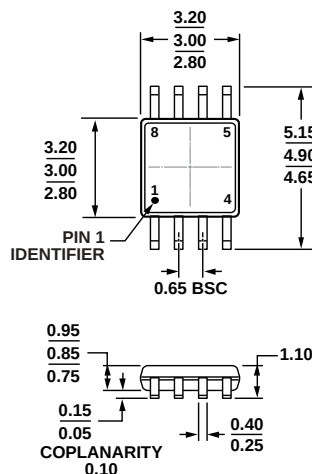
Figure 51. 8-Lead Mini Small Outline Package [MSOP] (RM-8)
