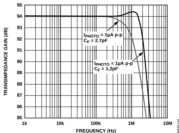
Figure 45. Photodiode Preamplifier Frequency Response
