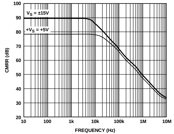
Figure 23. Common-Mode Rejection Ratio vs. Frequency
