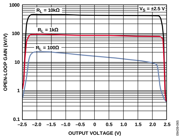
Figure 15. Open-Loop Gain vs. Output Voltage, V_S = \pm 2.5\text{ V}
