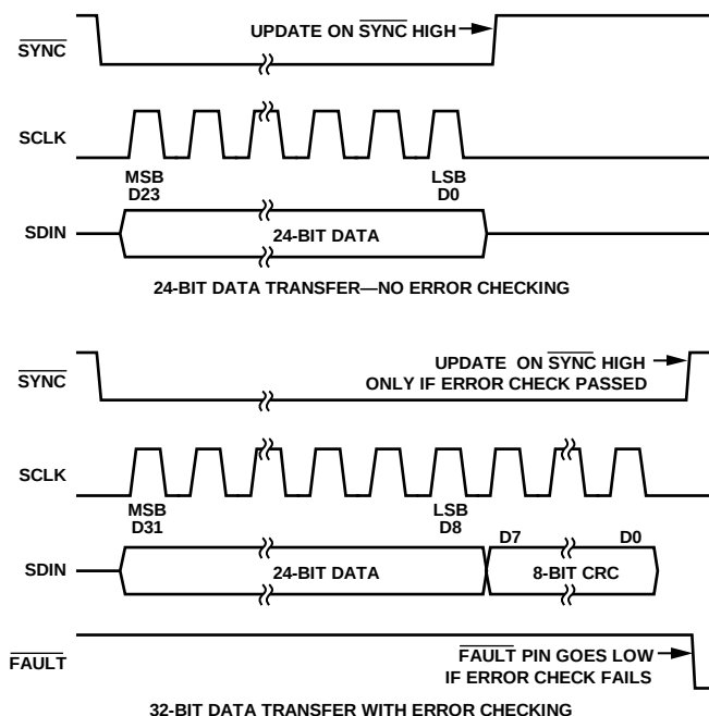
Figure 79. PEC Timing
