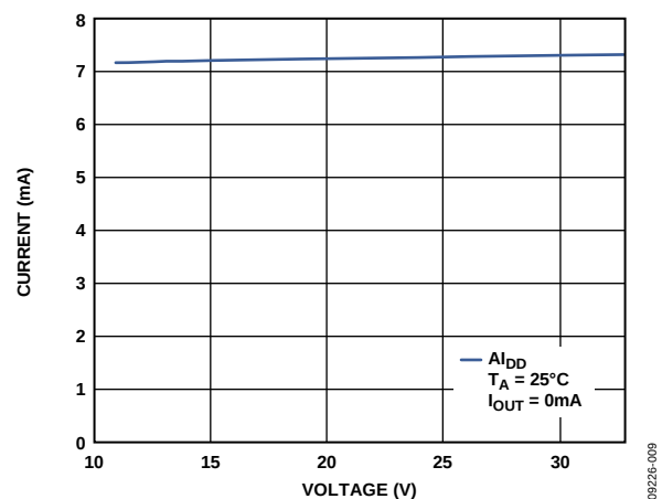
Figure 69. I_{DD} vs. AV_{DD}
