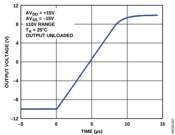
Figure 25. Full-Scale Positive Step
