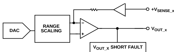
Figure 73. Voltage Output
