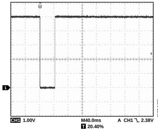
Figure 31. Typical Tactile Switch Characteristics
