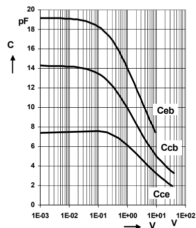
Capacitance
