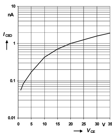
Dark Current
