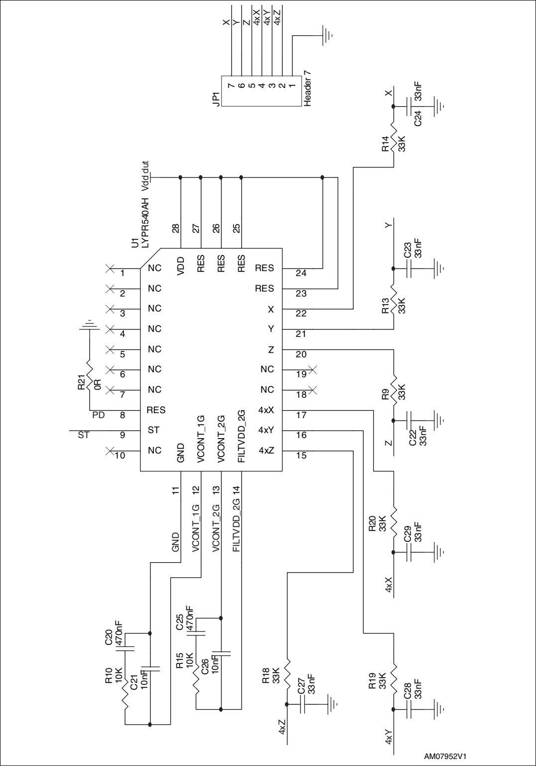
Figure 1. Sensor section
