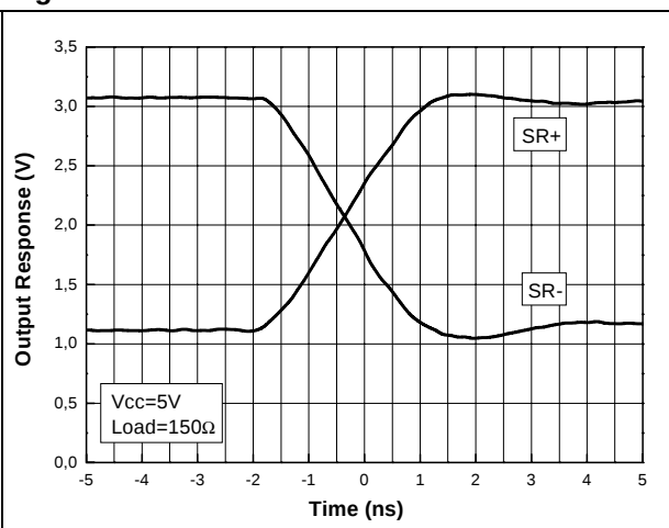
Figure 12. Slew rate
