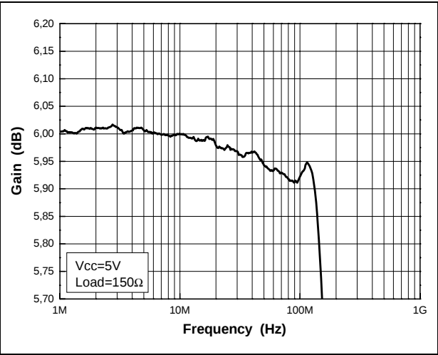
Figure 2. Gain flatness
