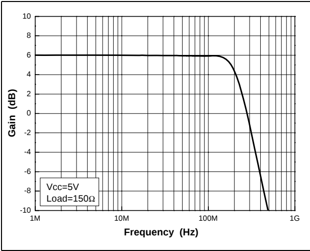
Figure 1. Frequency response
