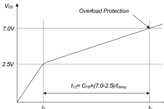
Figure 20. Overload Protection
