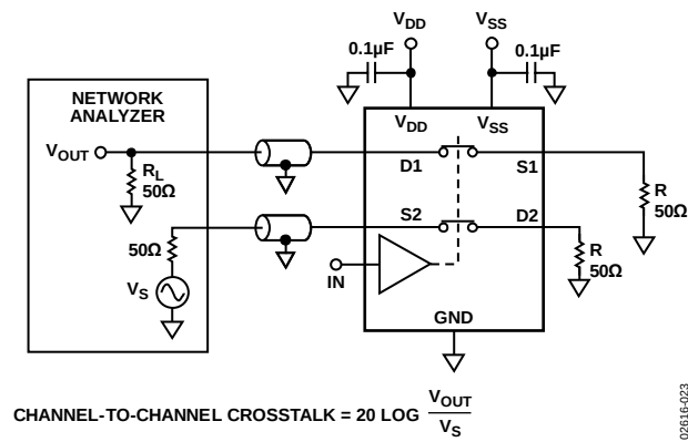
Figure 23. Channel-to-Channel Crosstalk
