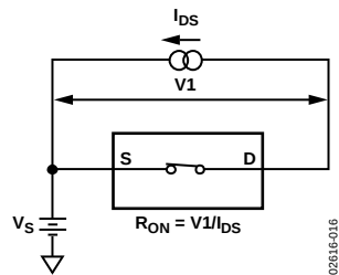
Figure 16. On Resistance
