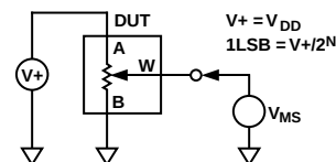
Figure 14. Potentiometer Divider Nonlinearity Error Test Circuit (INL, DNL)
