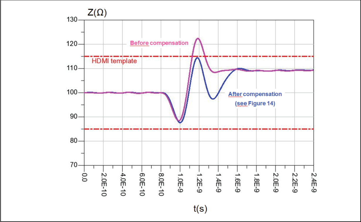
Figure 11. TDR
