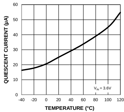
Quiescent Current vs. Temperature (MIC94162/3)
