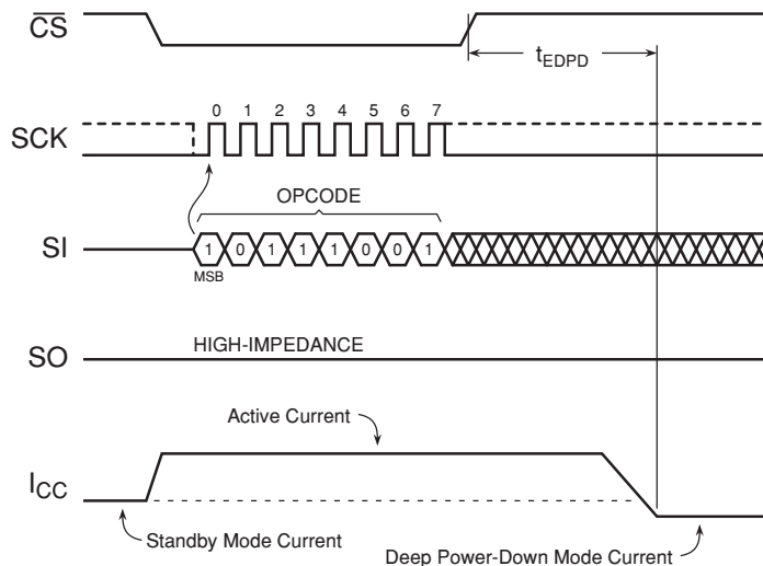
Figure 12-3. Deep Power-Down
