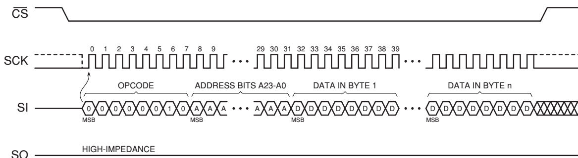
Figure 8-2. Page Program
