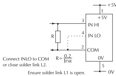
Measuring current. Meter power supply must be isolated from 4-20mA current loop.
