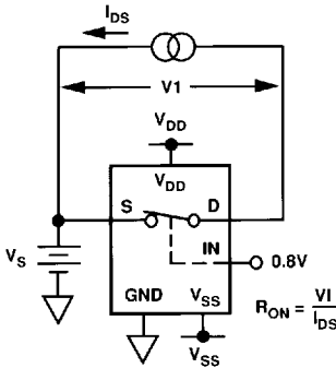
TEST CIRCUIT 1
