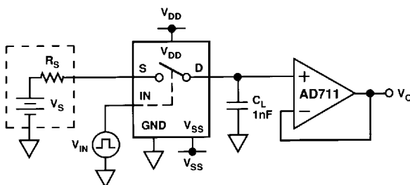
TEST CIRCUIT 7
