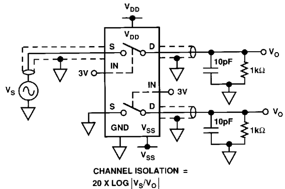
TEST CIRCUIT 6
