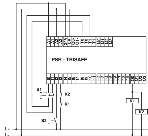
Application drawing
