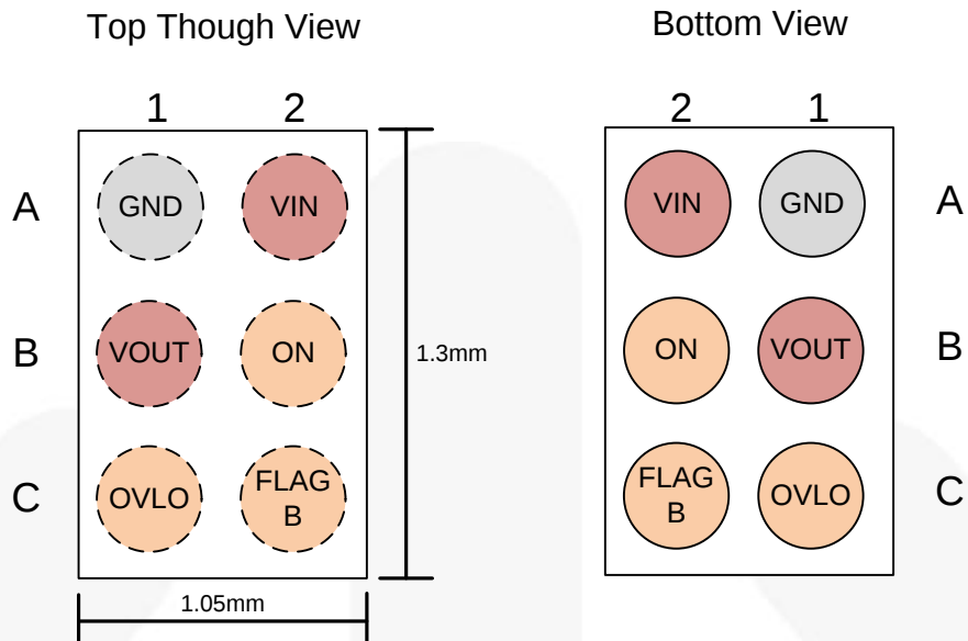
Figure 2. Pin Assignments
