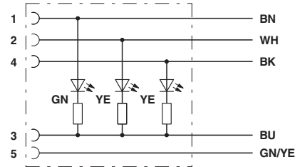
Contact assignment of M12 sockets with 3 LEDs
