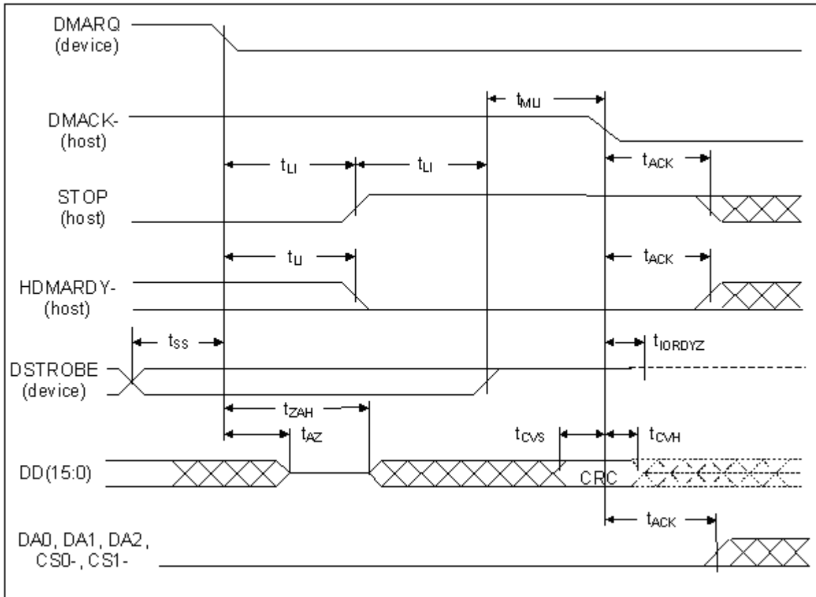
Device terminating an Ultra DMA data-in burst
