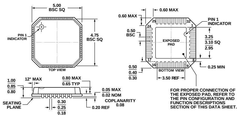
Figure 59. 32-Lead Lead Frame Chip Scale Package [LFCSP_VQ] 5 mm × 5 mm Body, Very Thin Quad (CP-32-2) Dimensions shown in millimeters
